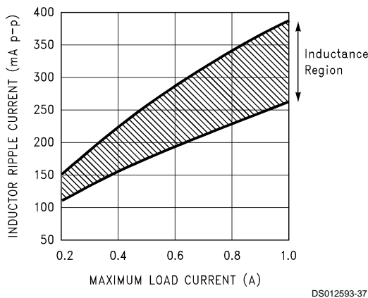
FIGURE 20. Peak-to-Peak Inductor Ripple Current vs Load Current
