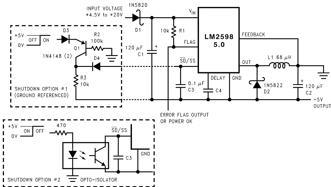
FIGURE 26. Inverting -5V Regulator With Shutdown and Soft-start
