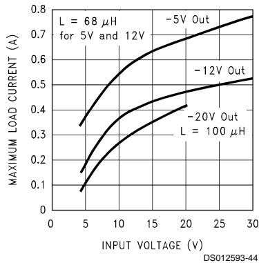
FIGURE 27. Maximum Load Current for Inverting Regulator Circuit
