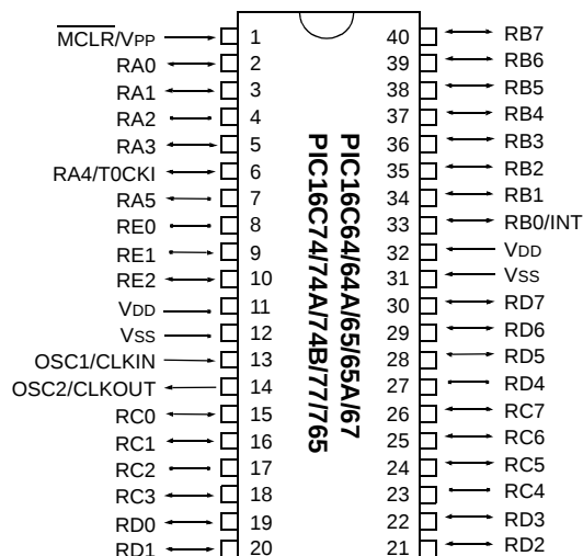
PDIP, Windowed Cerdip
