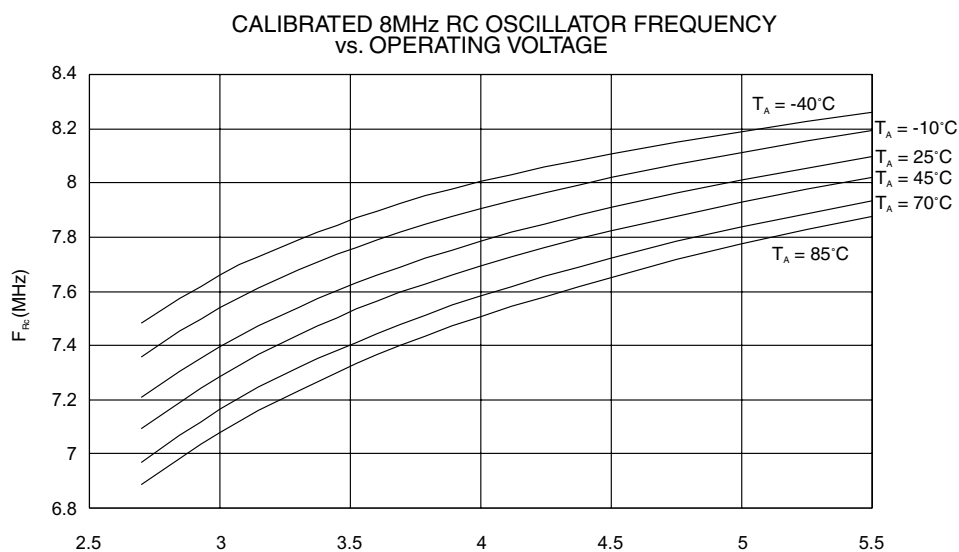
Figure 156. RC Oscillator Frequency vs. Operating Voltage (the devices are calibrated to 8 MHz at V_{CC} = 5V , T = 25^{\circ}C )
