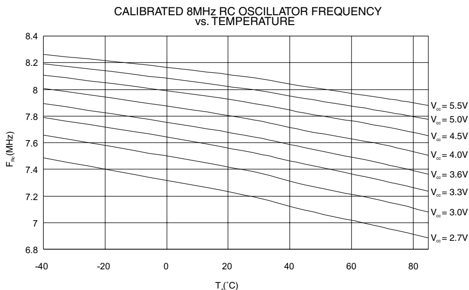
Figure 155. RC Oscillator Frequency vs. Temperature (the devices are calibrated to 8 MHz at V_{CC} = 5V , T = 25^{\circ}C )
