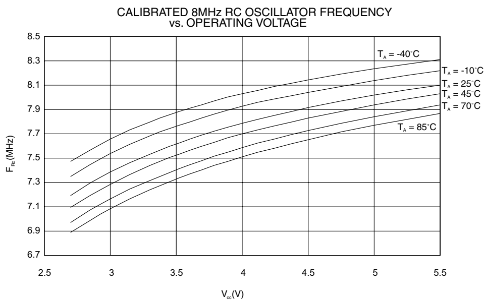
Figure 164. RC Oscillator Frequency vs. Operating Voltage (the devices are calibrated to 8 MHz at V_{cc} = 5V , T = 25^{\circ}C )
