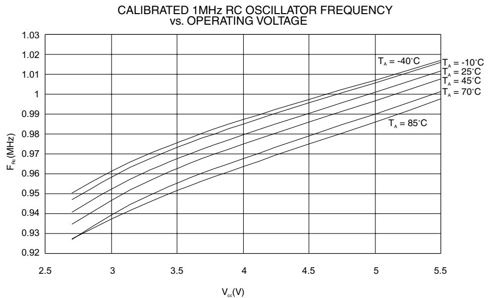
Figure 158. RC Oscillator Frequency vs. Operating Voltage (the devices are calibrated to 1 MHz at V_{cc} = 5V , T=25^{\circ}C )
