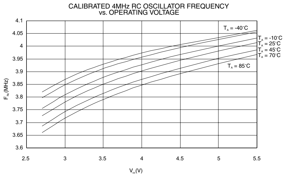
Figure 162. RC Oscillator Frequency vs. Operating Voltage (the devices are calibrated to 4 MHz at V_{cc} = 5V , T=25^{\circ}C )
