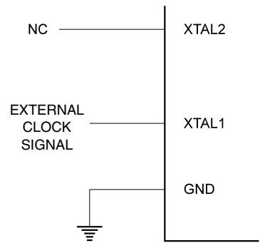
Figure 14. External Clock Drive Configuration
