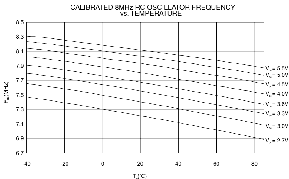
Figure 163. RC Oscillator Frequency vs. Temperature (the devices are calibrated to 8 MHz at V_{cc} = 5V , T = 25^{\circ}C )
