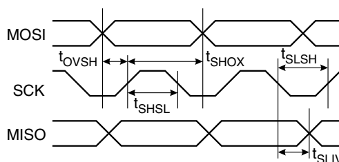
Figure 138. SPI Serial Programming Timing
