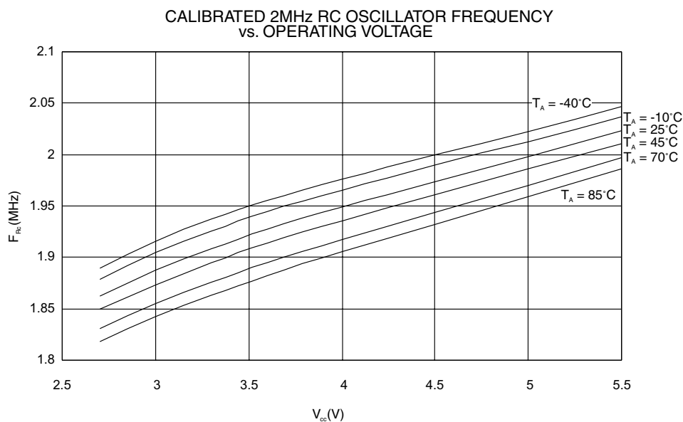
Figure 152. RC Oscillator Frequency vs. Operating Voltage (the devices are calibrated to 2 MHz at V_{cc} = 5V , T=25^{\circ}C )
