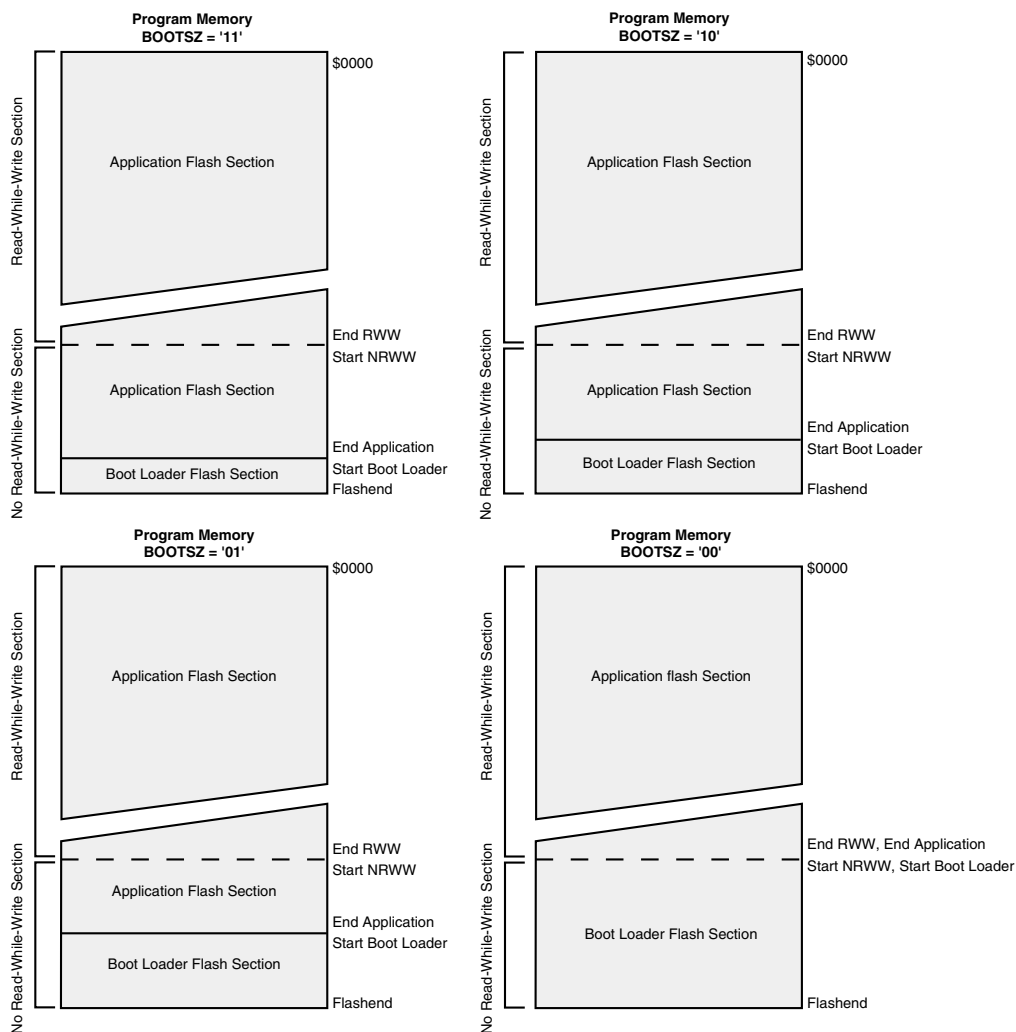
Figure 102. Memory Sections (1)
