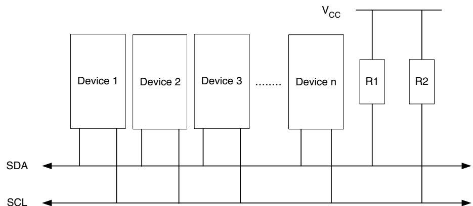
Figure 68. TWI Bus Interconnection
